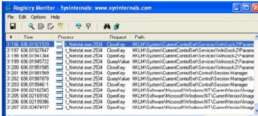
Figure 7: A Regmon Listing
