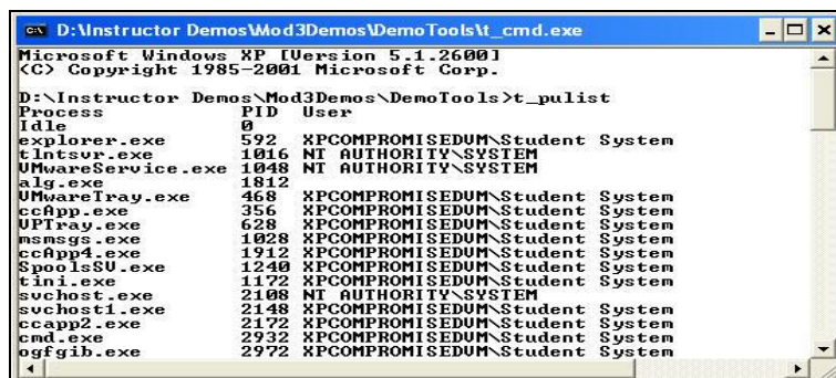
Figure 22: Pulist Output
