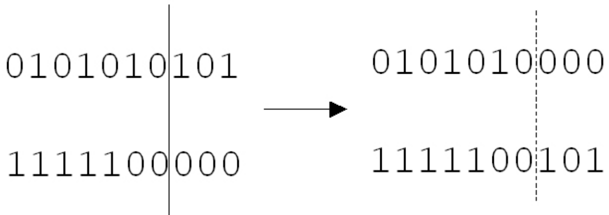
Figure 4.2 Crossover operation
